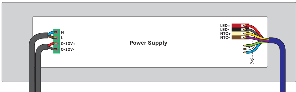
Connections to the Power Supply Unit of the MONO underwater light (inlc. 0-10Vdc dimmer)
